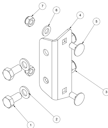
2103198 Lock Pin Bracket Kit
