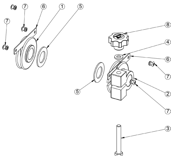
2103197 Bushing and Brake Kit
